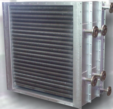
Steam to Air for Air Heater SUS 304 Fin and Tube
